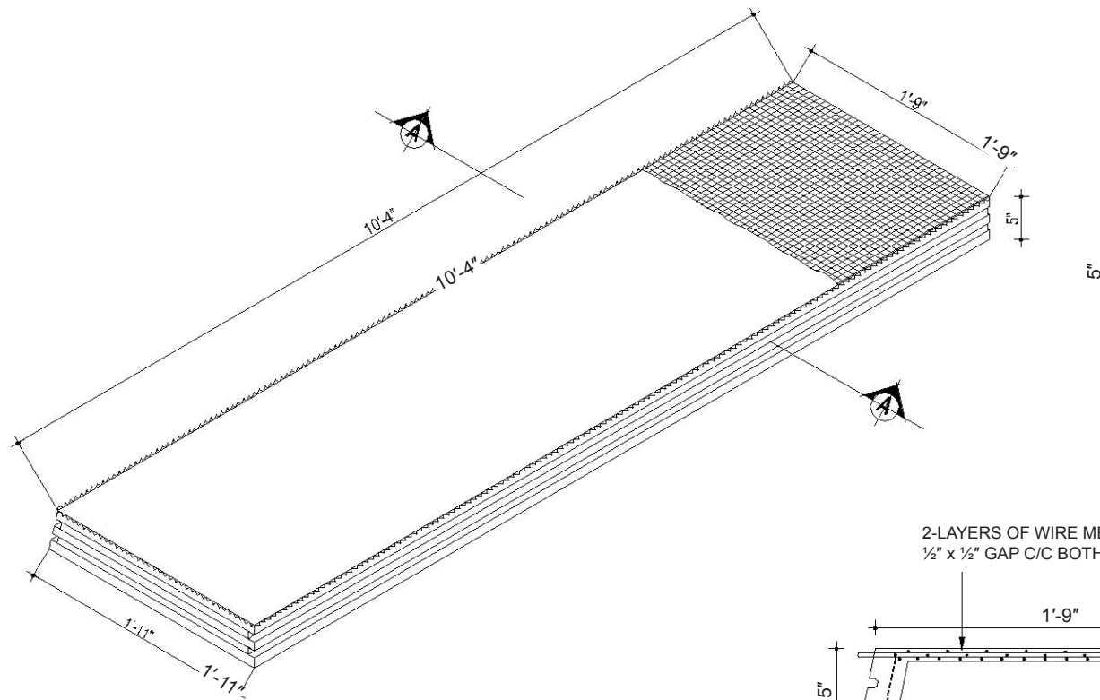
Isometric View of F. C. Channel
