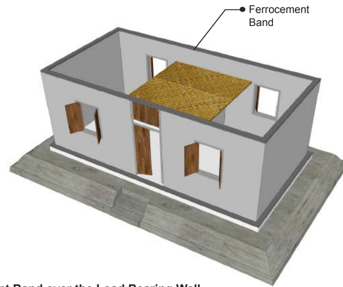
Ferrocement Band over the Load Bearing Wall
