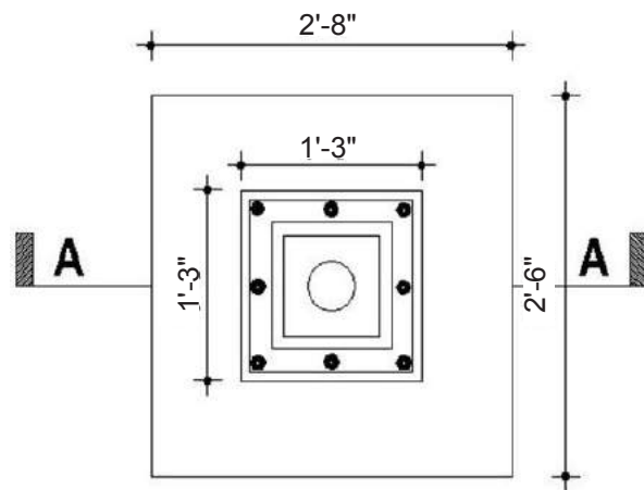
Plan of Precast (F.C.) Pocket Footing F-1
