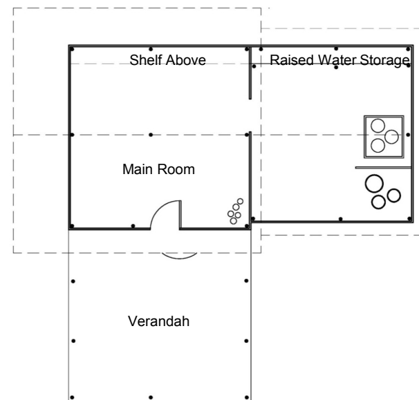
Typical House Plan of Marma Community
