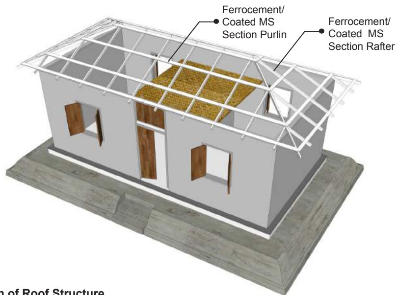
Addition of Roof Structure
