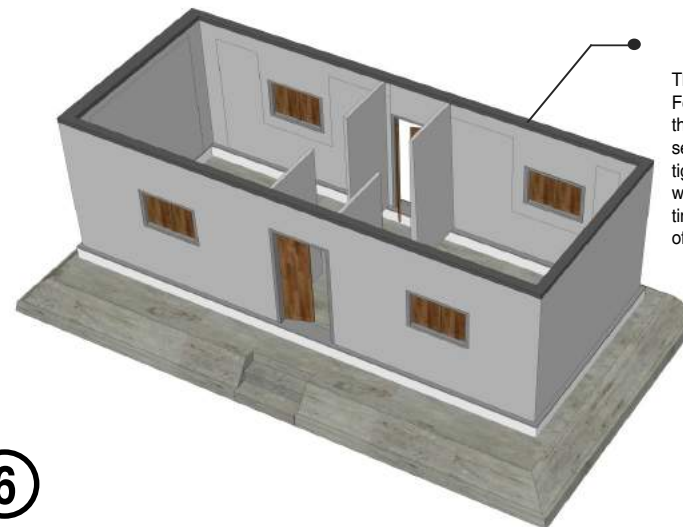
Superstructure with Ferrocement Band
