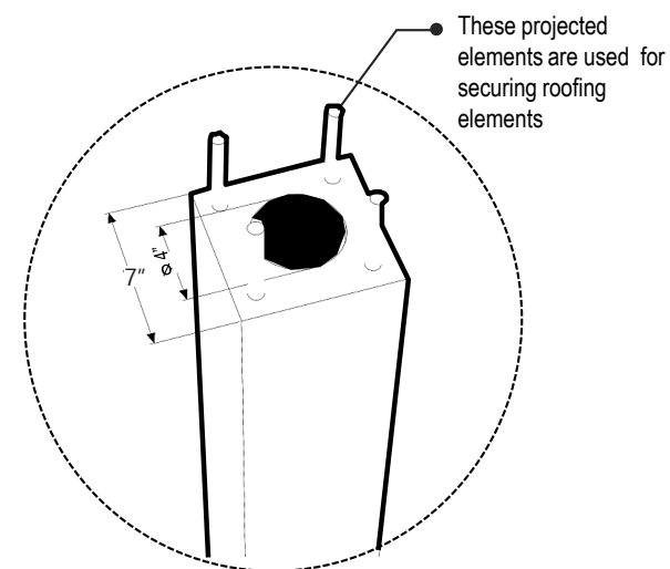
2 Blow up of Column Head
