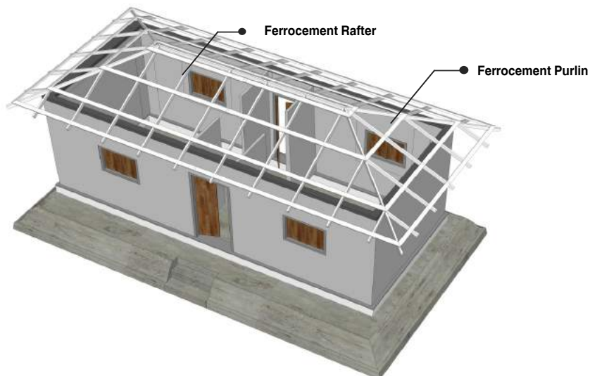
Superstructure with Roofing
