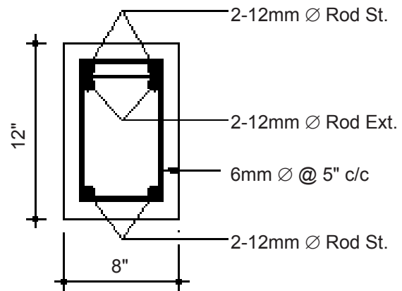
End Section of Beam B-1
