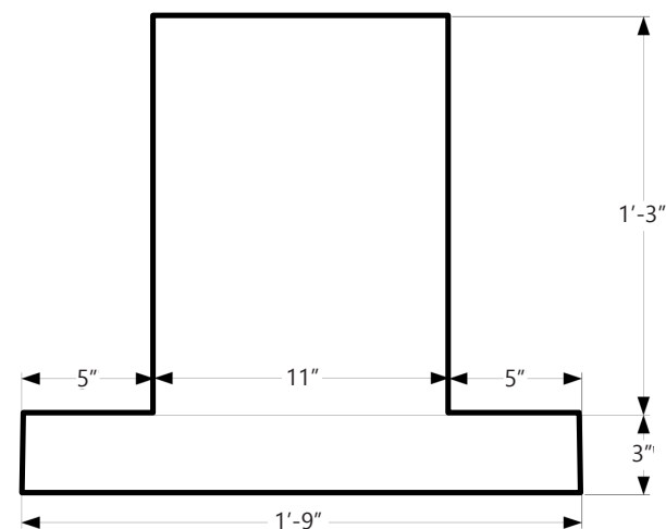
Elevation of stump pad footing
