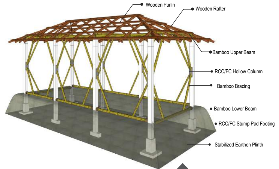
Hipped (Chouchala) Roof Structural Frame with Timber
