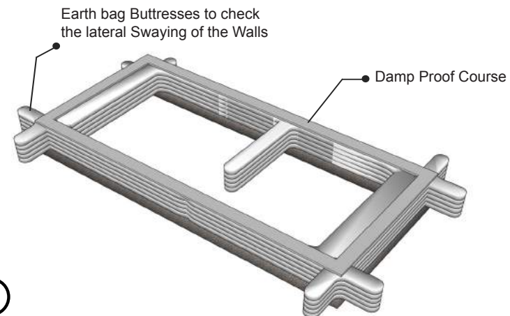
Damp Proof Course Erected upon the Gravel and Earth bag Foundation
