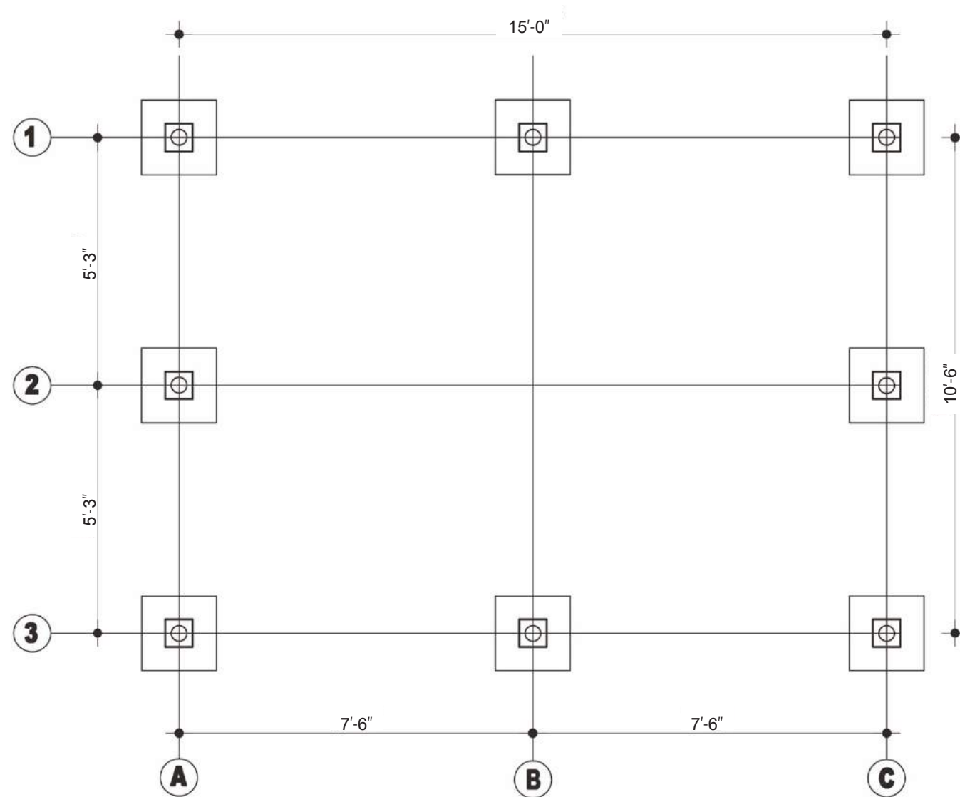
Foundation layout (Type 2)
