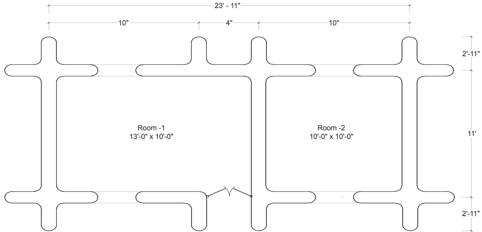
Floor plan
