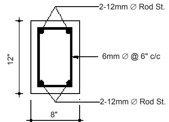
Mid Section of Beam B-2
