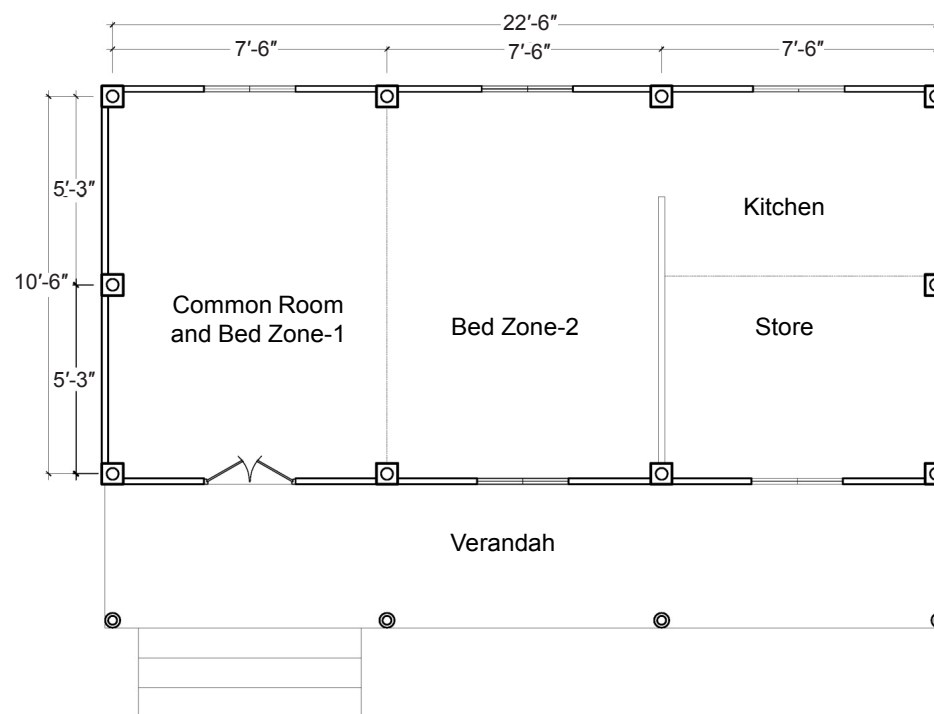
Plan with Additional Verandah
