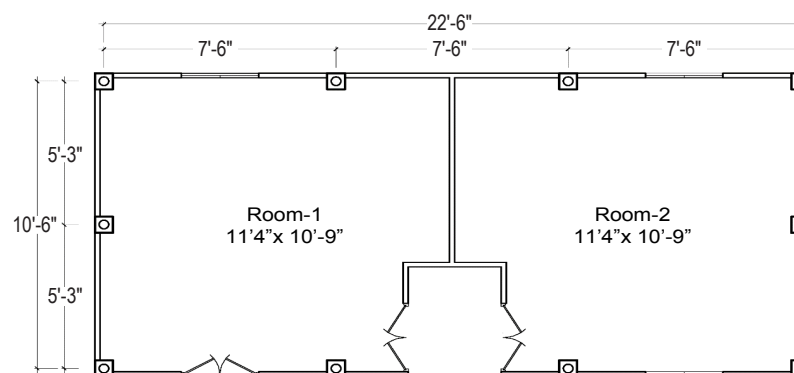
Plan ( Arrangement 4_for two families)
