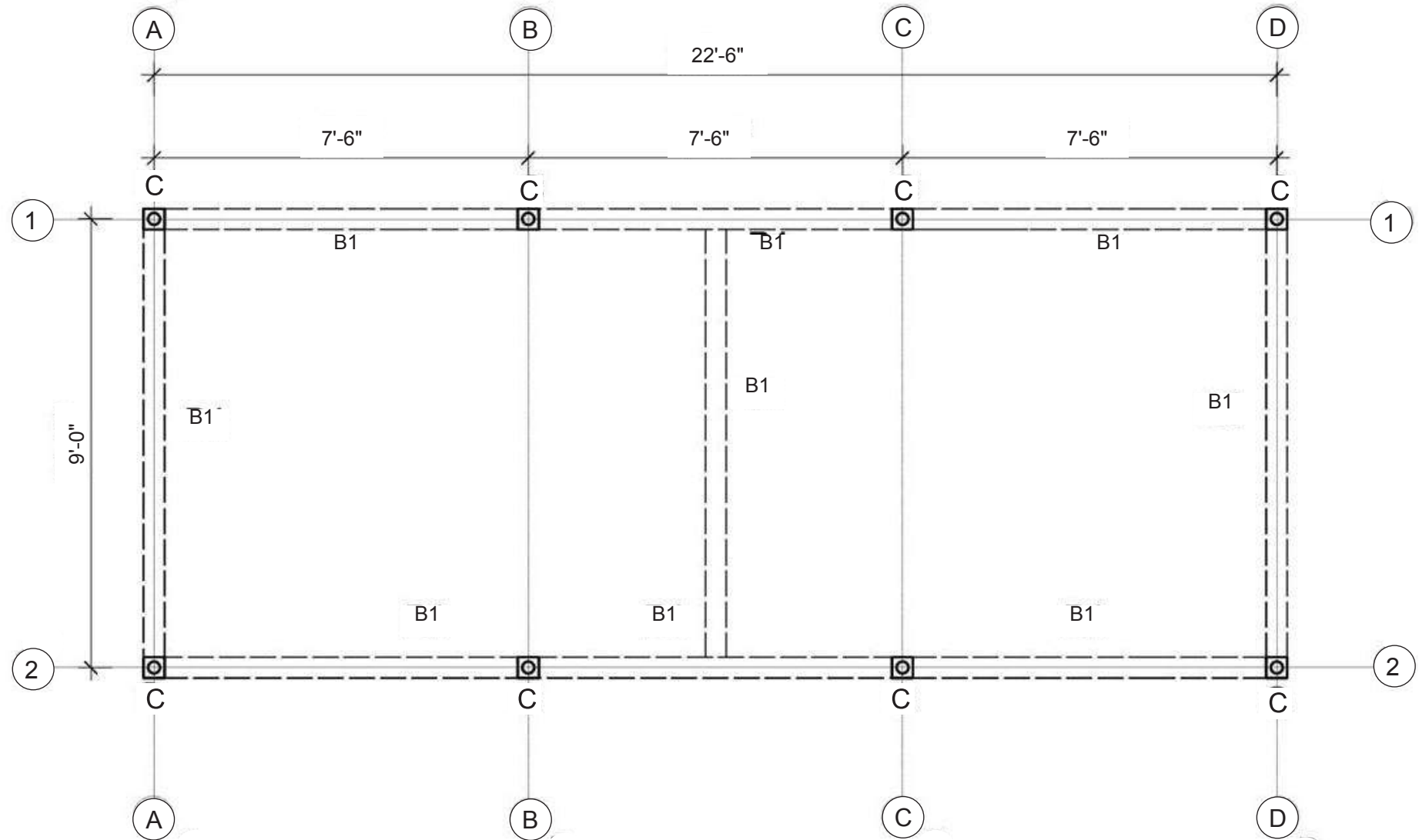
Beam-Column layout
