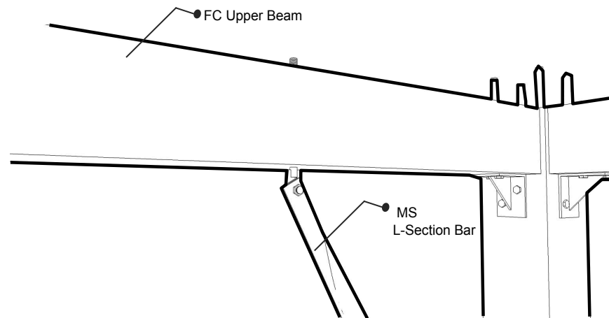
(27) Secure Assemblage of MS L-section and MS Bolted Joint Elements
