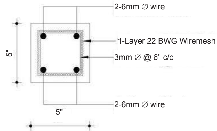
Section of Lintel
