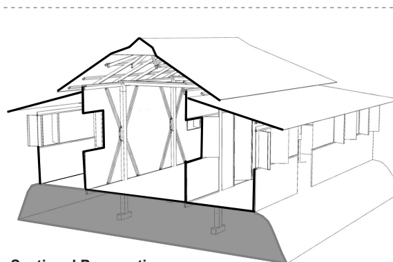
Sectional Perspective
