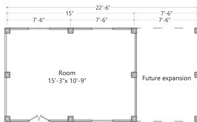
Expansion plan
