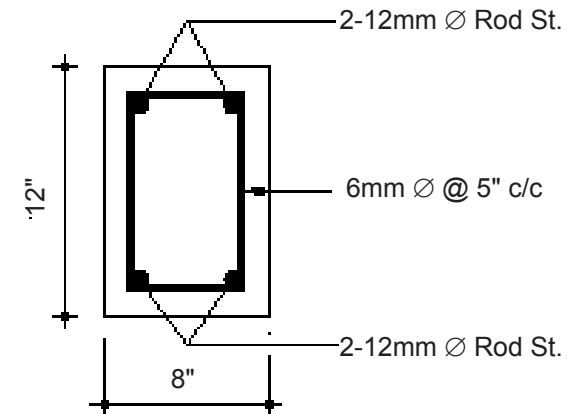
End Section of Beam B-2
