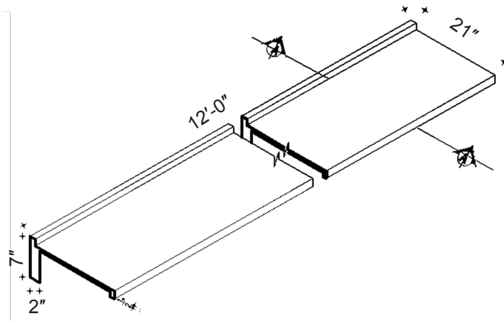
Isometric View
