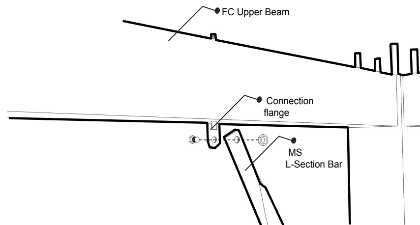
(26) Exploded View of MS L-section and MS Bolted Joint Elements
