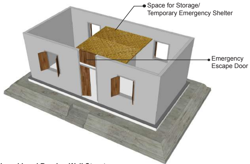
Plinth and Load Bearing Wall Structure
