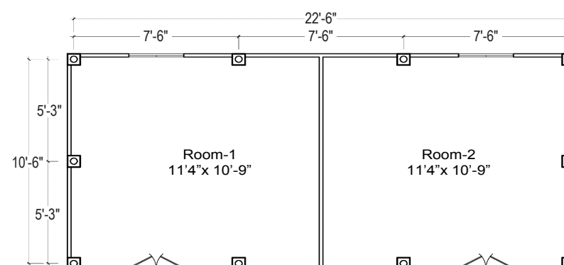
Plan ( Arrangement 2_for two families)
