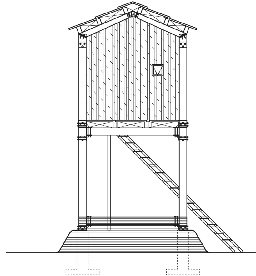
Side Elevation
