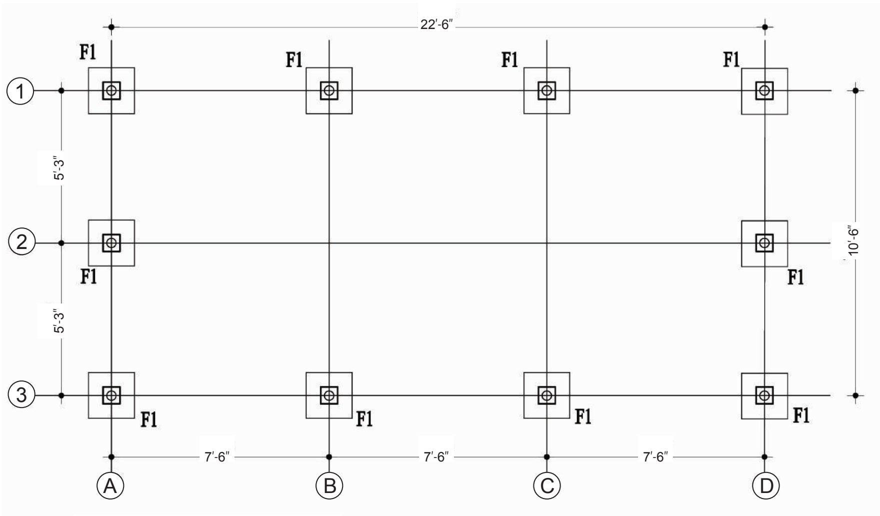
Foundation layout
