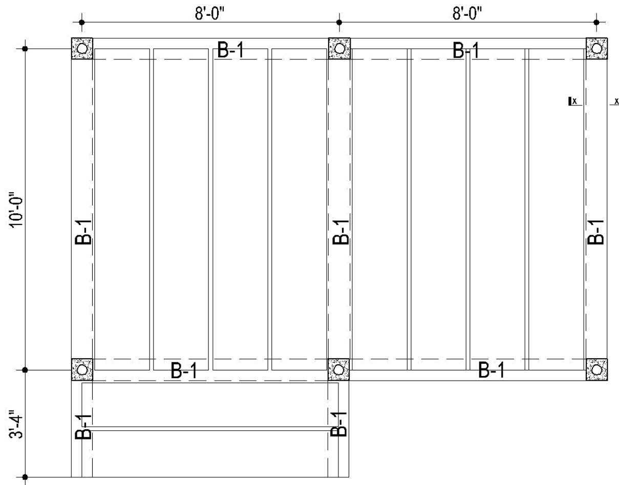
Floor Beam and Channel Arrangement
