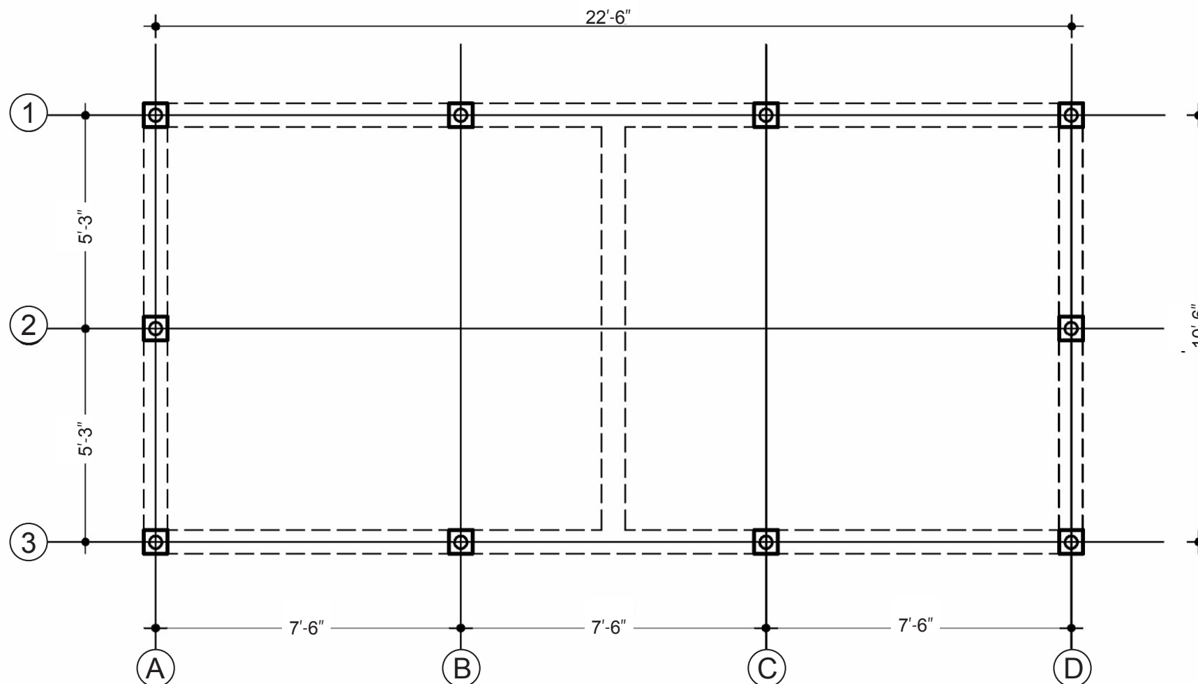
Beam-Column layout
