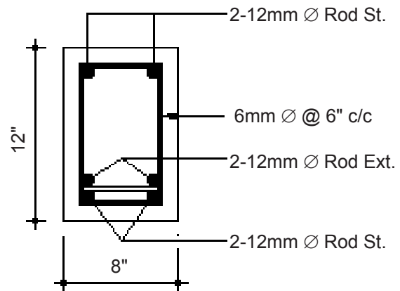
Mid Section of Beam B-1
